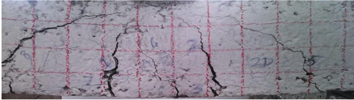
Fig. 13 - Deflection pattern of C40P3
