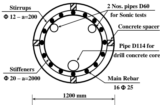
(a). Cross-section detail of Pile TP2
