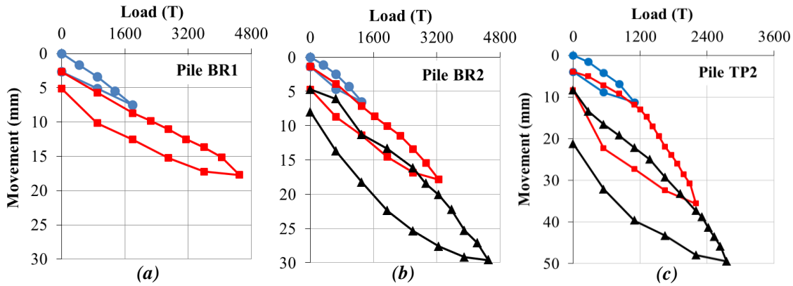
Fig.3 - Load – movement curves of three tested piles
