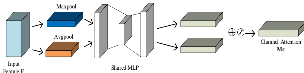
Fig. 4 - Structure of Channel Attention Module
